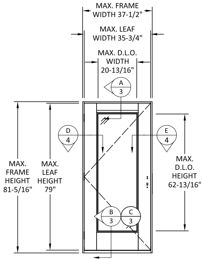
TYPICAL ELEVATION
