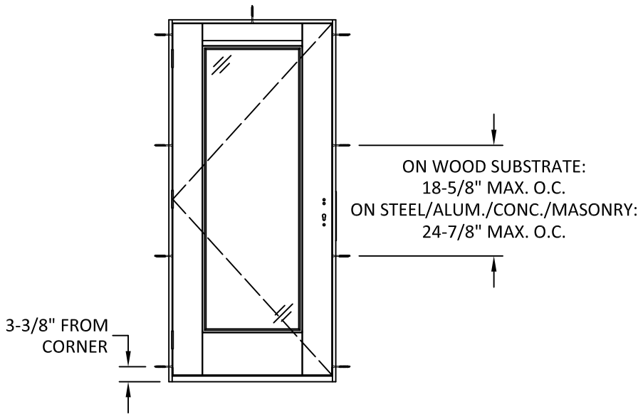
ANCHOR LAYOUT
